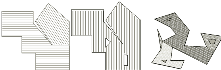
FIGURE 5.6 Examples of an optimized coverage path planning algorithm based on a headland turning cost function and a divide-and-conquer strategy for 2D terrains, where the inner polygons indicate nontraversable obstacles. (From Jin, J. and L. Tang. 2006. Optimal Path Planning for Arable Farming , ASABE Paper Number 061158, ASABE, St. Joseph, MI, USA; Jin, J. and L. Tang. 2010. Transactions of the ASABE , 53:283–295. With permission.)
