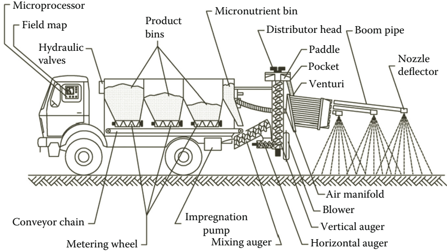
FIGURE 10.11 Design of a truck-mounted multibin fertilizer air spreader.
