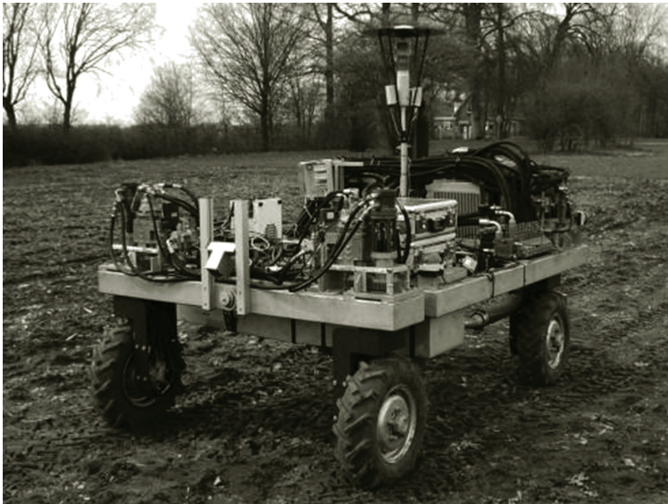
FIGURE 5.16 A weeding robot developed at Wageningen University. (From Bakker, T., J. Bontsema, and J. Müller. 2010a. Journal of Terramechanics , 47:63–73. With permission.)
